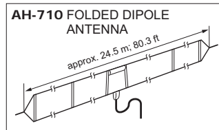
Covers from 1.9 to 30 MHz band. Has an SO-239 connector. Easy to assemble (non-kink construction).
