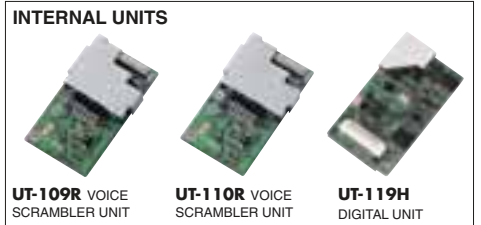
UT-109R : Non-rolling type voice scrambler. UT-110R : Rolling type voice scrambler. UT-119H : Digital unit. Provides 6.25kHz digital capability.
